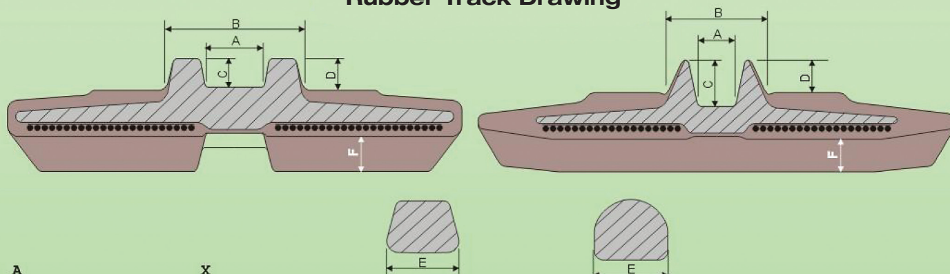
Rubber Track Drawing
