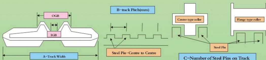
Track Size Identification
